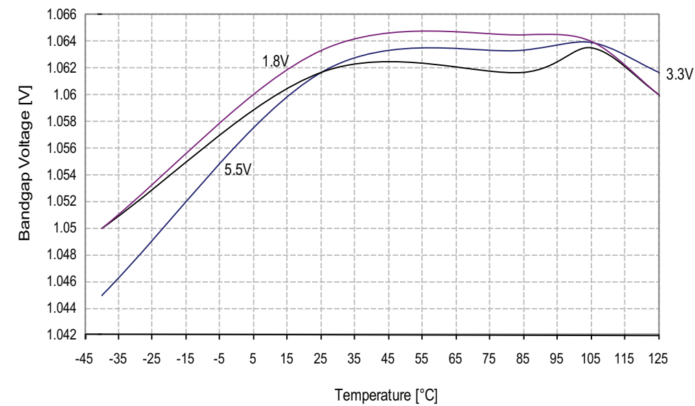
Figure 26-53. Bandgap Voltage vs. Temperature
