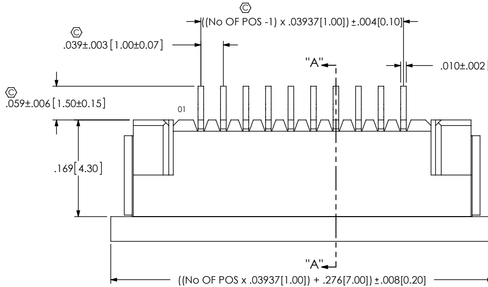
BACK VIEW
