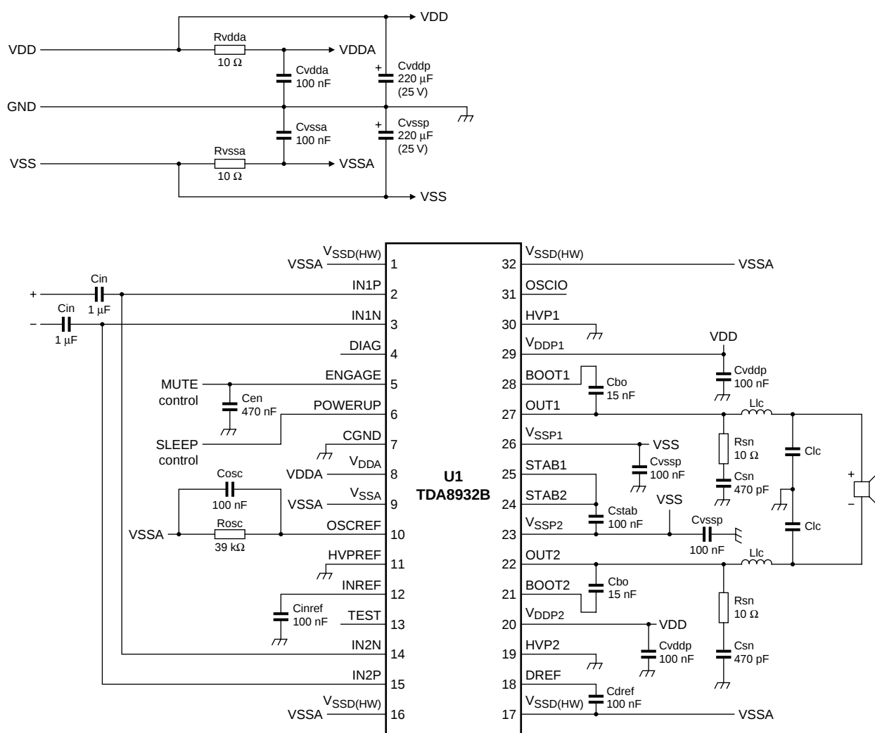
Fig 39. Typical simplified application diagram for 1 × BTL (symmetrical supply)
