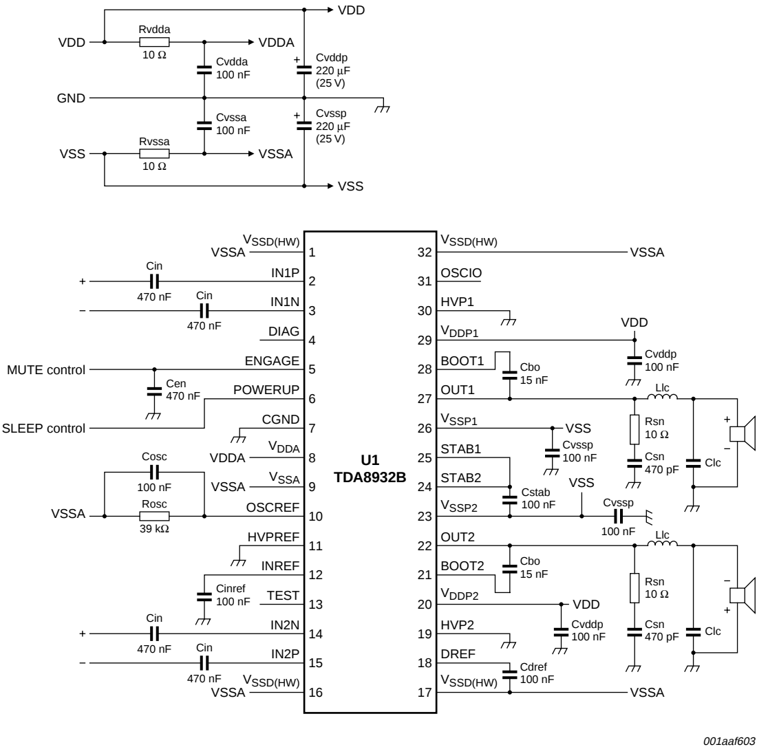
Fig 38. Typical simplified application diagram for 2 × SE (symmetrical supply)
