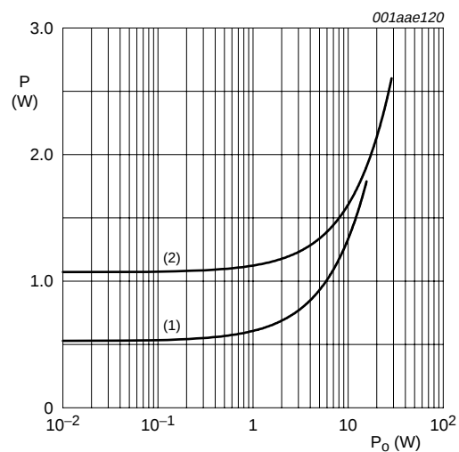
f_i = 1\ \text{kHz} ; power dissipation in junction only (1) V_P = 12\ \text{V} ; R_L = 4\ \Omega (2) V_P = 22\ \text{V} ; R_L = 8\ \Omega
