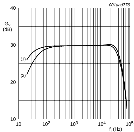
V_i = 100 \text{ mV (RMS)} ; R_i = 0 \text{ } \Omega ; C_{se} = 1000 \text{ } \mu\text{F} (1) V_P = 30 \text{ V} ; R_L = 2 \times 8 \text{ } \Omega (2) V_P = 22 \text{ V} ; R_L = 2 \times 4 \text{ } \Omega
