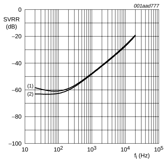
V_{\text{ripple}} = 500 \text{ mV (RMS)} referenced to ground; R_i = 0 \text{ } \Omega (shorted input) (1) V_P = 30 \text{ V} ; R_L = 2 \times 8 \text{ } \Omega (2) V_P = 22 \text{ V} ; R_L = 2 \times 4 \text{ } \Omega
