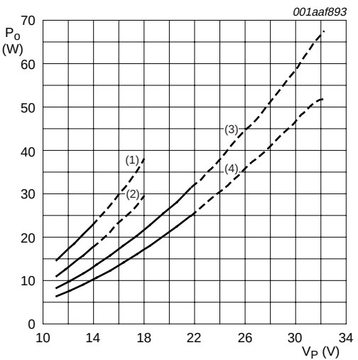
f_i = 1\text{ kHz} (short time P_O ); dashed line will require heat sink for continuous time output power (1) R_L = 4\ \Omega ; THD+N = 10 % (2) R_L = 4\ \Omega ; THD+N = 0.5 % (3) R_L = 8\ \Omega ; THD+N = 10 % (4) R_L = 8\ \Omega ; THD+N = 0.5 %
