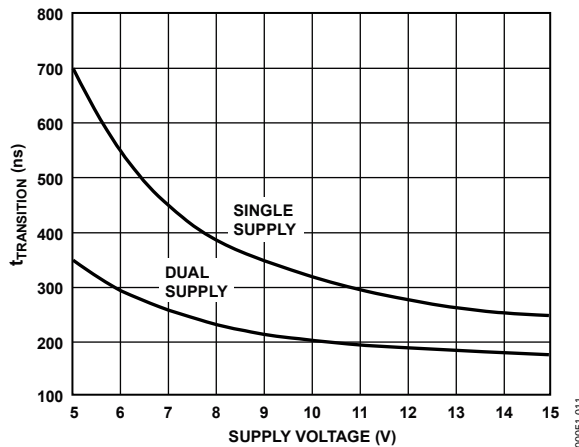
Figure 10. t_{TRANSITION} vs. Supply Voltage: Dual and Single Supplies, T_A = 25^\circ\text{C} (Note: For V_{DD} and V_{SS1} < 10\text{ V} ; V1 = V_{DD}/V_{SS1} , V2 = V_{SS}/V_{DD} . (see Figure 19))
