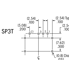
Right Angle PC Footprints
