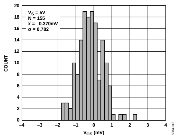
Figure 36. V_{OS} Distribution
