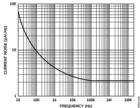
Figure 35. Current Noise vs. Frequency
