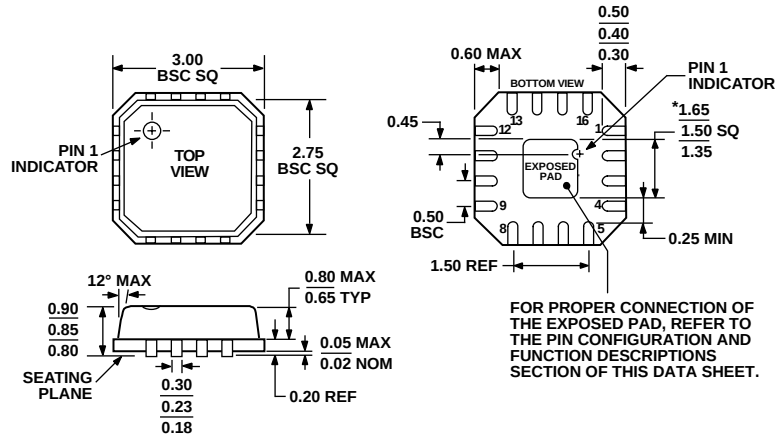
Figure 54. 16-Lead Lead Frame Chip Scale Package [LFCSP_VQ] 3 mm × 3 mm Body, Very Thin Quad (CP-16-3) Dimensions shown in millimeters
