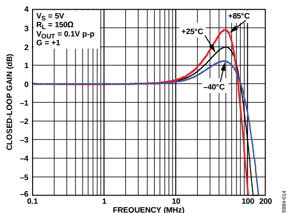
Figure 16. Small Signal Frequency Response for Various Temperatures
