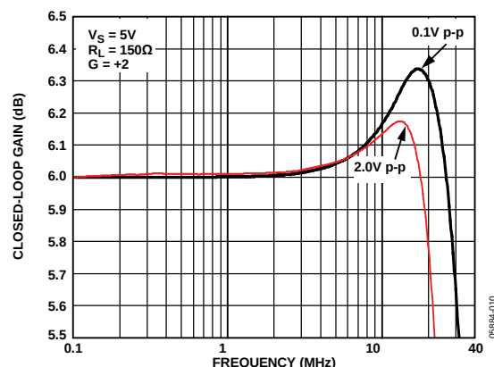
Figure 5. 0.5 dB Flatness Frequency Response
