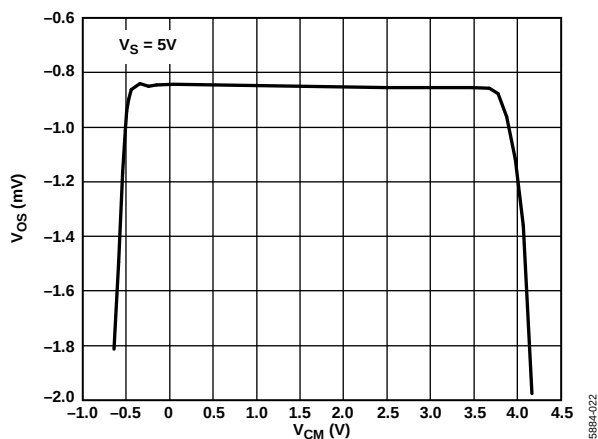
Figure 50. V_{OS} vs. Common-Mode Voltage, V_S = 5\text{ V}
