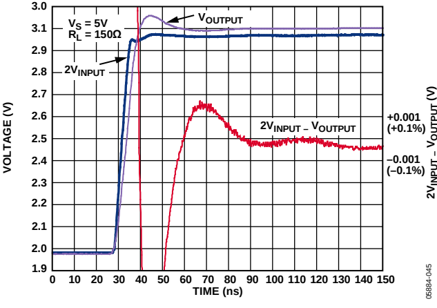
Figure 46. 0.1% Settling Time
