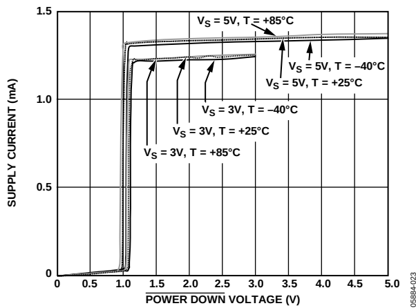
Figure 38. Supply Current vs. POWER DOWN Voltage
