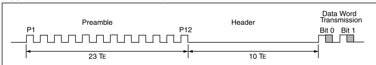
FIGURE 7-2: PREAMBLE/HEADER FORMAT
