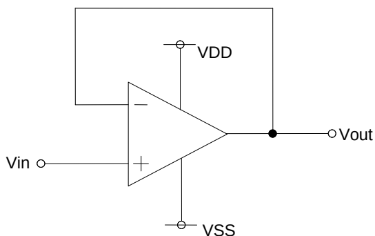
Fig.167 voltage follower circuit
