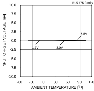
Fig.152 Input Offset Voltage – Ambient Temperature ( V_{cm}=V_{DD}-1.2[V] , V_{OUT}=1.5[V] )
