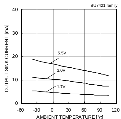
Fig.127 Output Sink Current - Ambient Temperature (VOUT=VSS+0.4[V])
