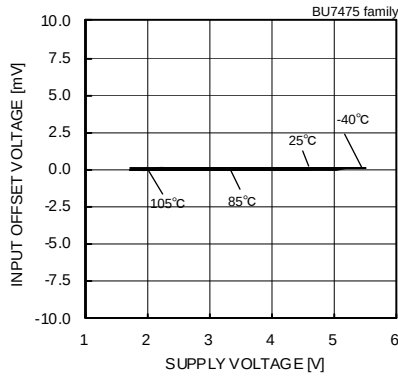
Fig.151 Input Offset Voltage – Supply Voltage ( V_{cm}=V_{DD}-1.2[V] , V_{OUT}=1.5[V] )
