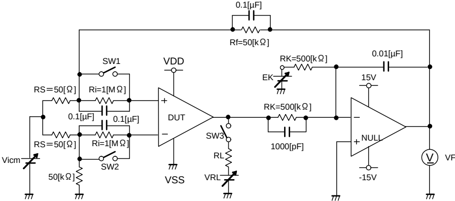
Fig.163 Test circuit 1
