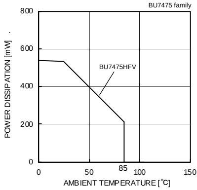
Derating curve
