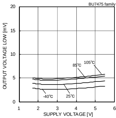
Output Voltage Low – Supply Voltage ( R_L=10[k\Omega] )
