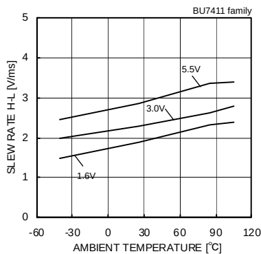
Fig.114 Slew Rate H-L – Ambient Temperature
