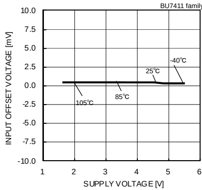
Fig.105 Input Offset Voltage – Supply Voltage ( V_{icm}=V_{DD}-1.2[V] , V_{OUT}=1.5[V] )
