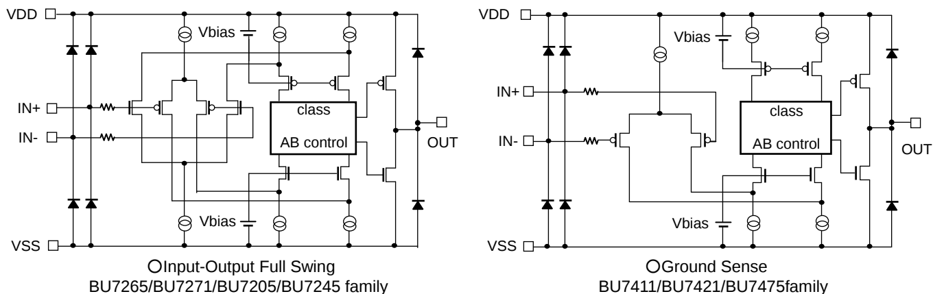
Fig.162 Schematic Diagram
