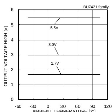
Fig.121 Output Voltage High - Ambient Temperature (RL=10[kΩ])
