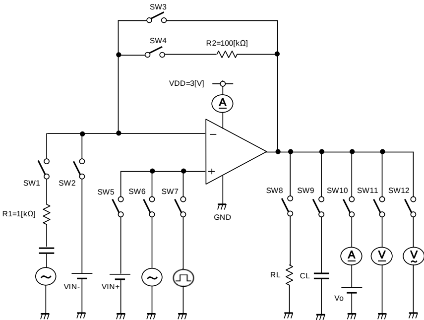
Fig.164 Test circuit 2
