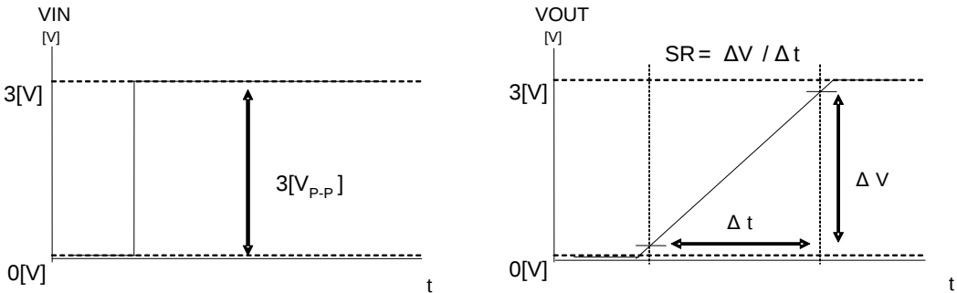
Fig.165 Slew rate input output wave (Input-Output Full Swing BU7261/BU7271/BU7205/BU7245 family)
