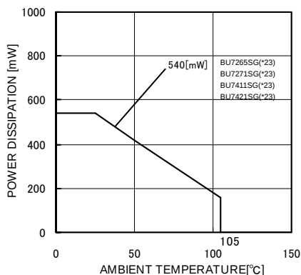
(e) BU7265SG BU7271SG BU7411SG BU7421SG
