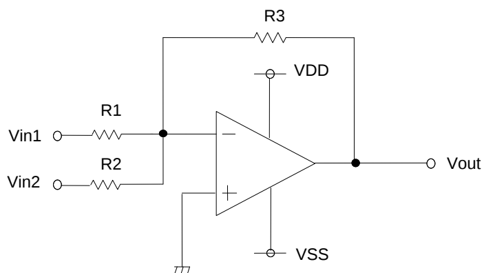
Fig.170 Adder circuit
