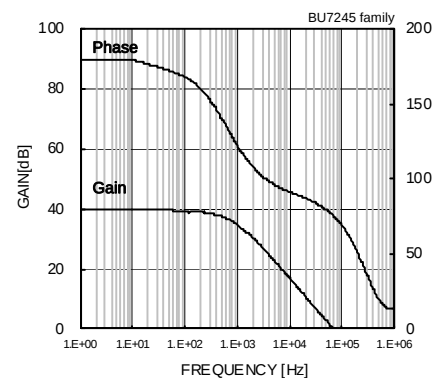
Fig.92 Gain – Frequency
