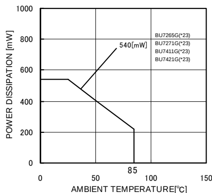
(c) BU7265G BU7271G BU7411G BU7421G
