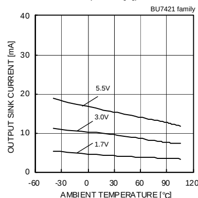
Fig.127 Output Sink Current - Ambient Temperature (VOUT=VSS+0.4[V])
