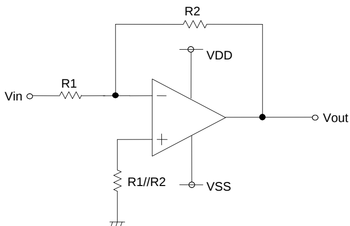
Fig.168 Inverting amplifier circuit
