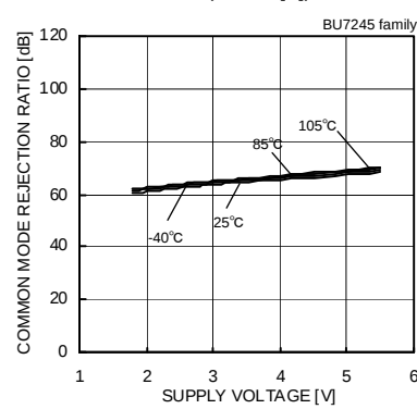
Fig.87 Common Mode Rejection Ratio – Supply Voltage
