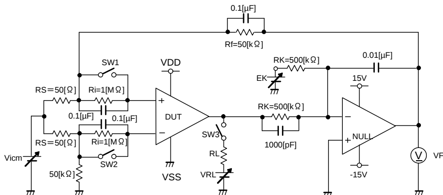
Fig.163 Test circuit 1
