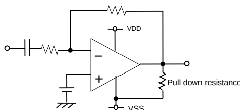
Fig.174 Pull down resistance
