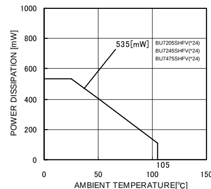
(f) BU7205SHFV BU7245SHFV BU7475SHFV
