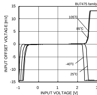
Fig.153 Input Offset Voltage – Input Voltage ( V_{DD}=3[V] )
