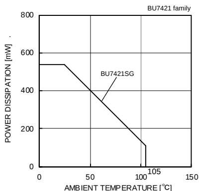
Fig.117 Derating curve
