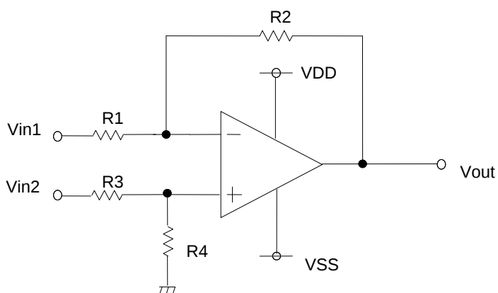
Fig.171 Differential amplifier
