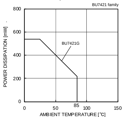
Fig.116 Derating curve
