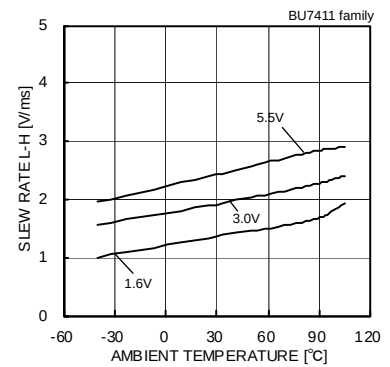
Fig.113 Slew Rate L-H – Ambient Temperature
