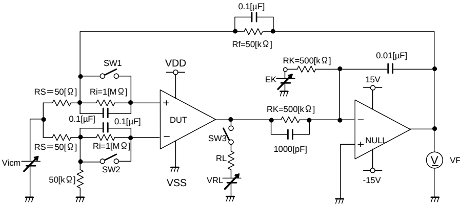
Fig.163 Test circuit 1
