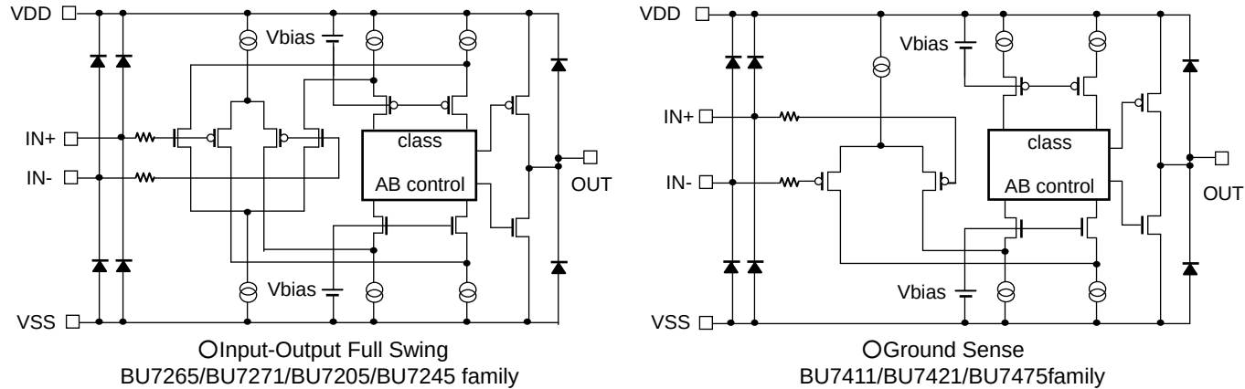
Fig.162 Schematic Diagram
