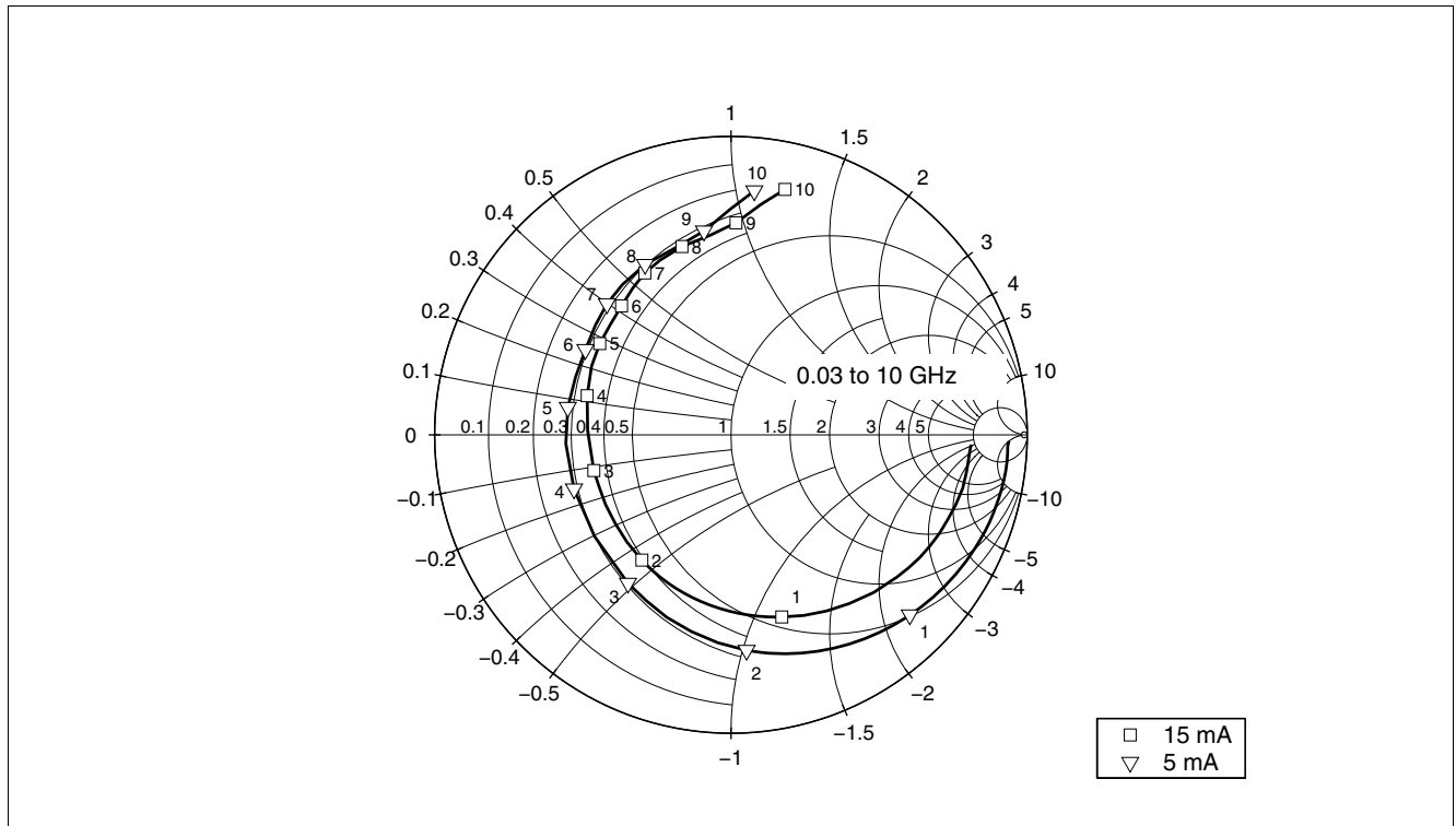
Figure 14 Input Matching S_{11} = f(f) , V_{CE} = 3 V, I_C = 5 / 15 mA
