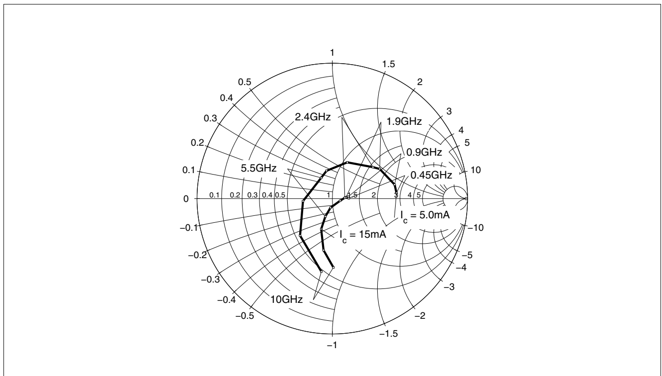
Figure 15 Source Impedance for Minimum Noise Figure Z_{opt} = f(f) , V_{CE} = 3 V, I_C = 5 / 15 mA
