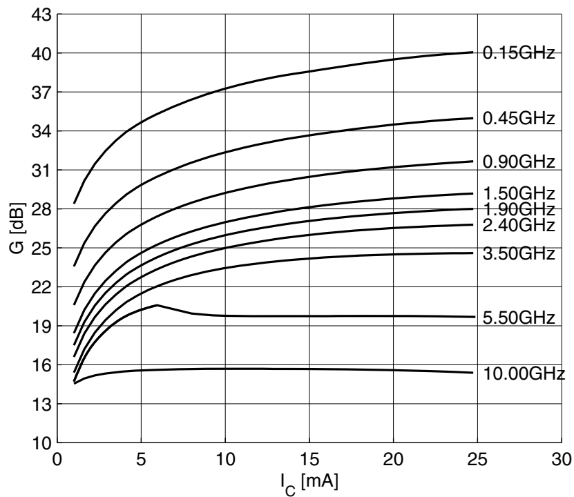
Figure 12 Maximum Power Gain G_{\max} = f(I_C) , V_{CE} = 3V , f = Parameter in GHz
