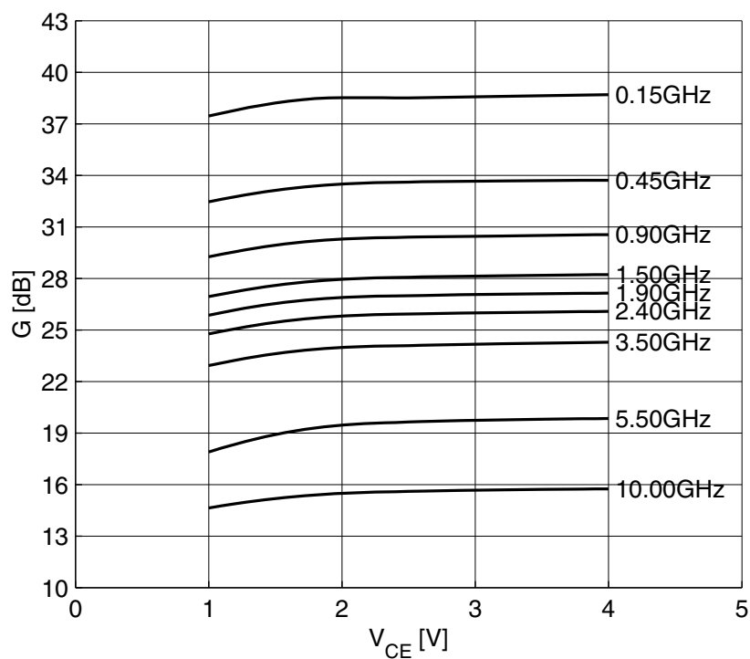
Figure 13 Maximum Power Gain G_{\max} = f(V_{CE}) , I_C = 15mA , f = Parameter in GHz
