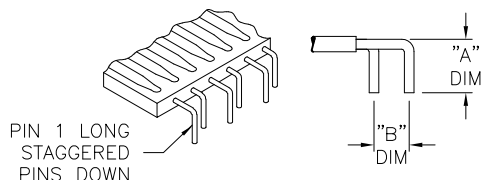
G BEND RIGHT ANGLED STAGGERED PINS DOWN
