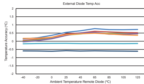
Figure 2-2. Temperature Accuracy vs. Remote Diode Temperature, V_{DD} = 1.8\text{V}
