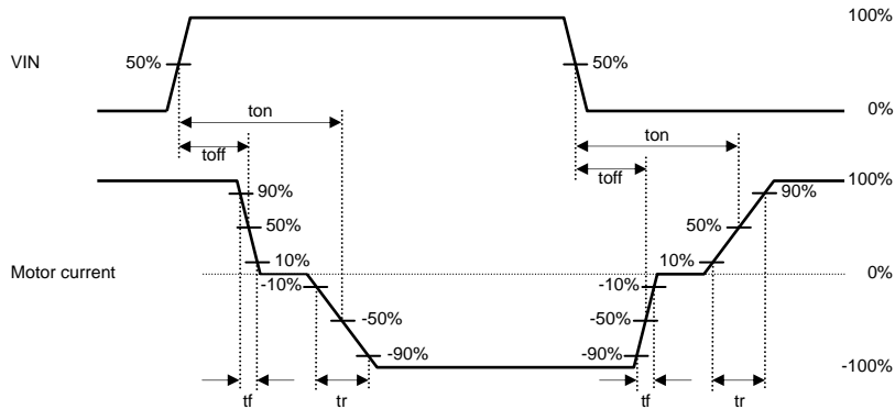
Fig.6 BD6886GUL, BD6369GUL I/O Switching Waveform
