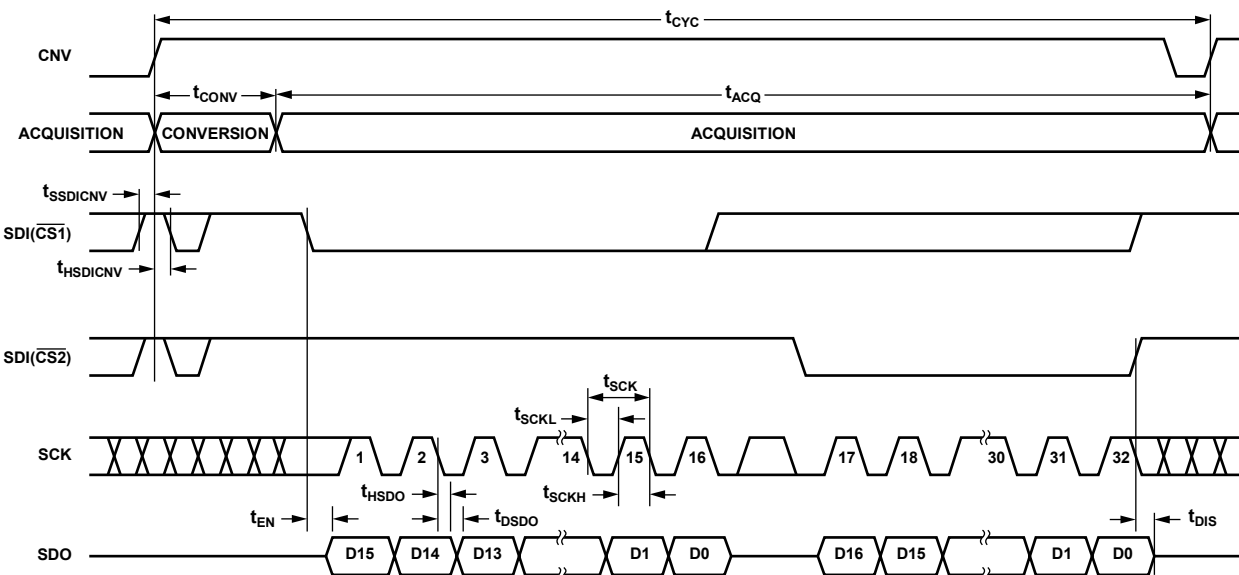
Figure 38. \overline{\text{CS}} Mode, 4-Wire Without Busy Indicator Serial Interface Timing
