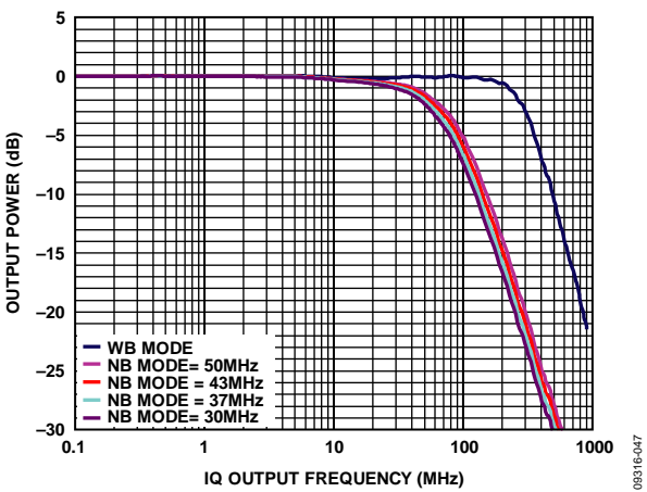
Figure 43. Normalized IQ Output Bandwidth, Narrow-Band, and Wideband Modes, Nominal Conditions
