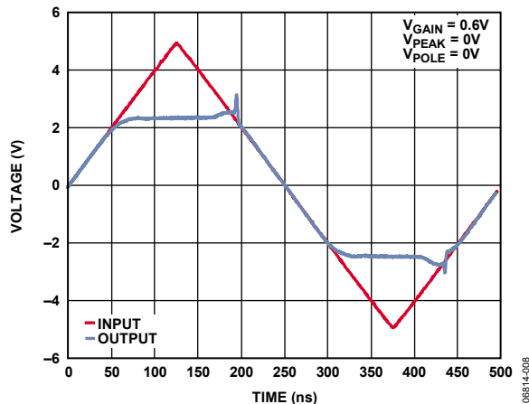
Figure 10. Overdrive Recovery
