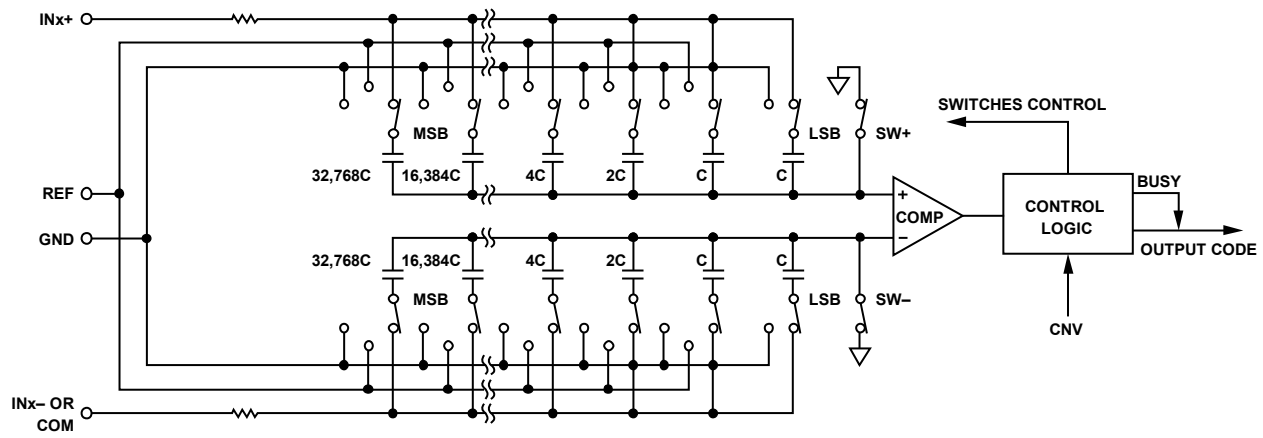
Figure 25. ADC Simplified Schematic
