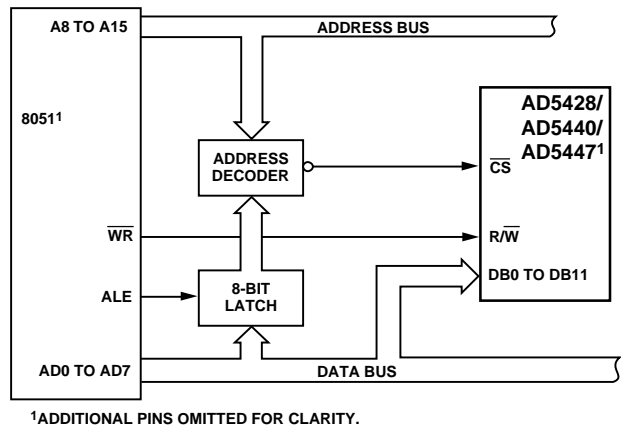
Figure 45. 8xC51-to-AD5428/AD5440/AD5447 Interface
