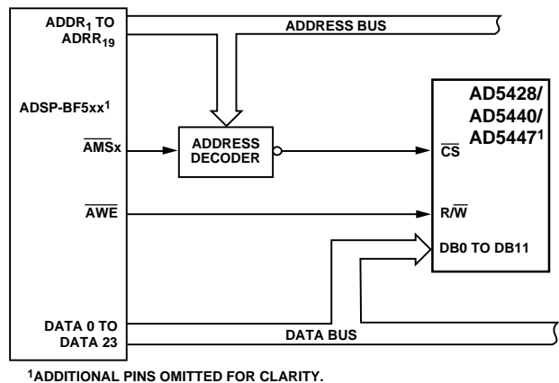
Figure 46. ADSP-BF5xx-to-AD5428/AD5440/AD5447 Interface
