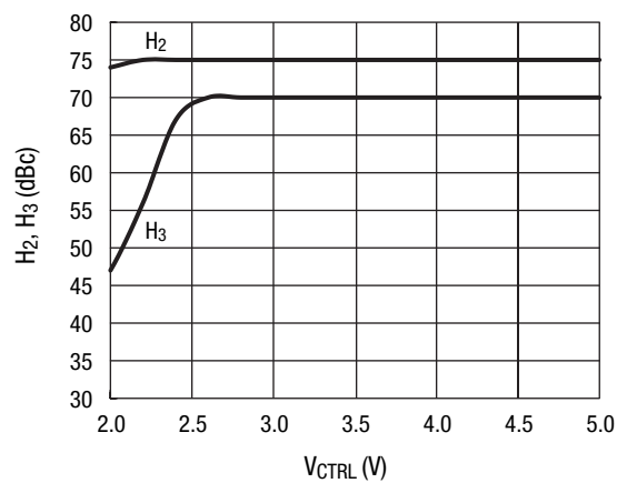
Second and Third Harmonics vs. Control Voltage f_{IN} = 900 \text{ MHz} , P_{IN} = 34.5 \text{ dBm} , GSM Signal
