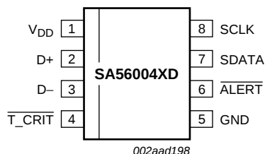
Fig 2. Pin configuration for SO8
