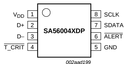
Fig 3. Pin configuration for TSSOP8
