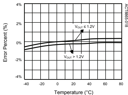
REG4, 5, 6, 7 Output Voltage vs. Temperature
