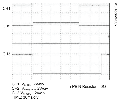
Manual Reset Response
