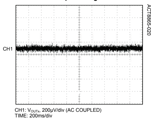
LDO Output Voltage Noise
