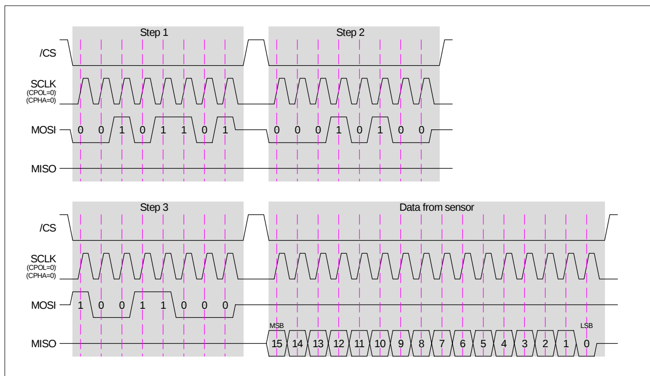
Fig. 5: SPI data transfer
