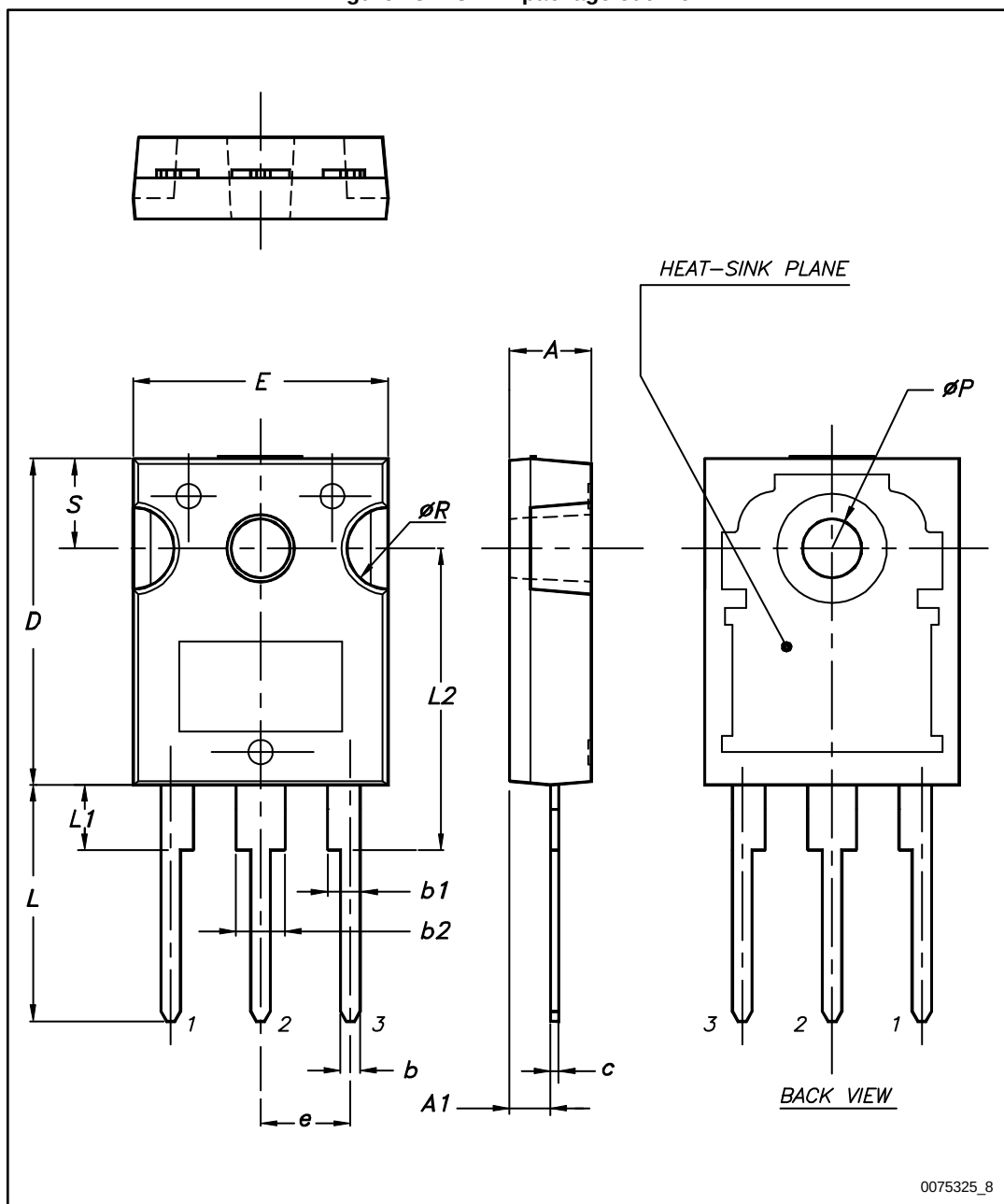
Figure 23: TO-247 package outline
