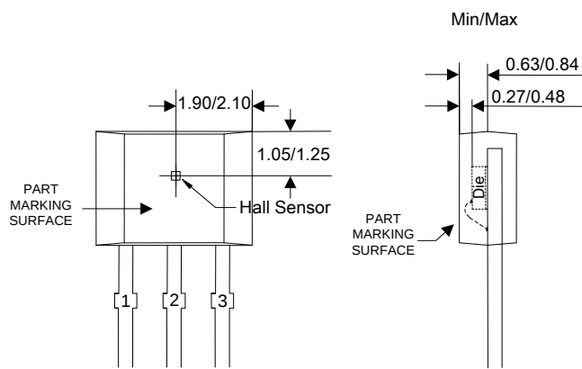
Sensor Location
