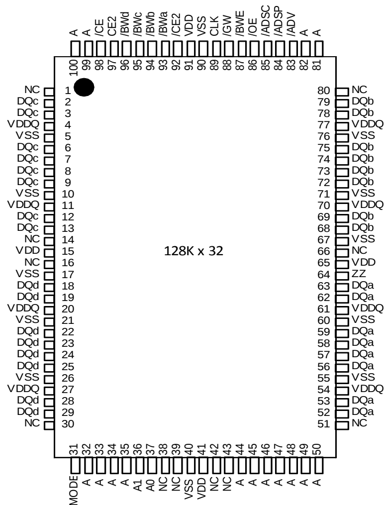
128K x 32, 100PIN QFP (Top View)
