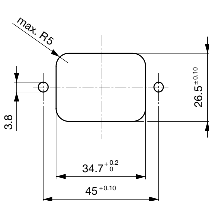
Panel cut-out and Drilling diagram
