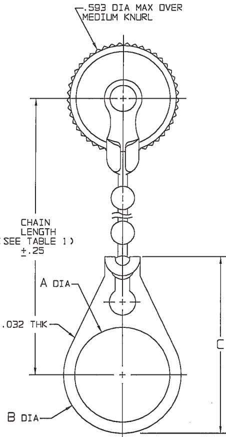
-2- A -D1 THRU -11- A -DD8 SHOWN STANDARD CHAIN AND BULKHEAD JACK MOUNTING LUG
