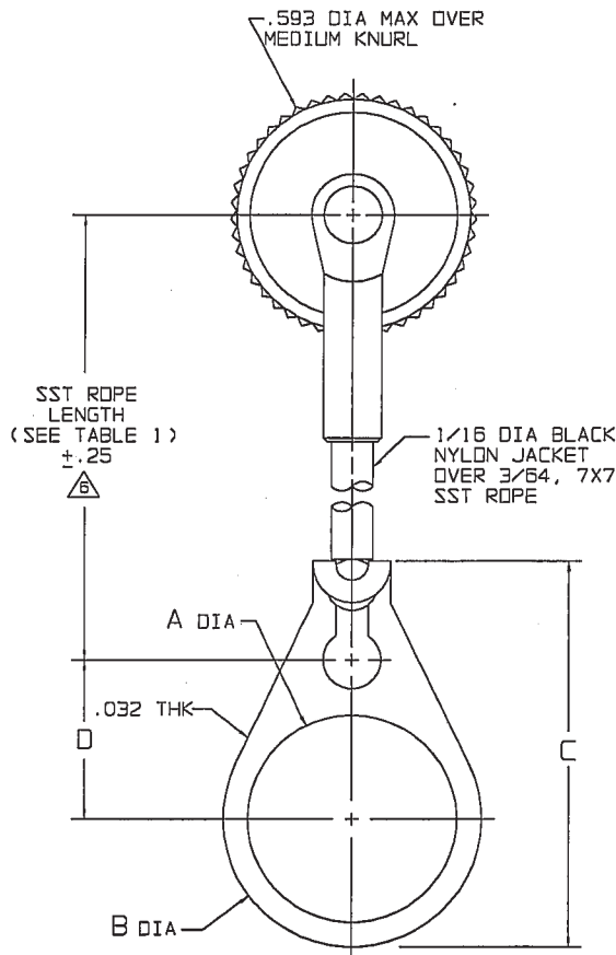
-12- A -D1 THRU -17- A -DD8 SHOWN STAINLESS STEEL ROPE AND BULKHEAD JACK MOUNTING LUG
