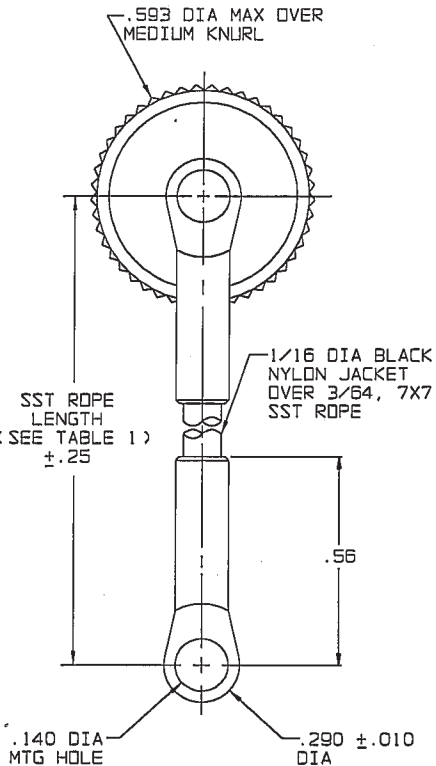
-12- A THRU -17- A SHOWN STAINLESS STEEL ROPE AND MOUNTING LUG
