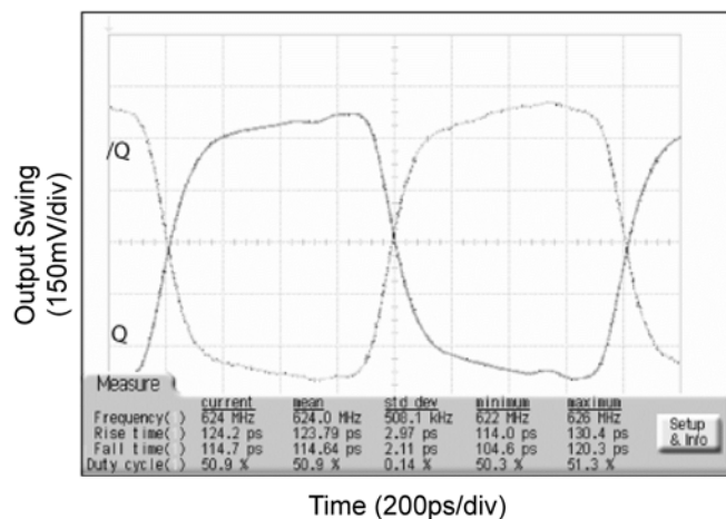
622MHz Output
