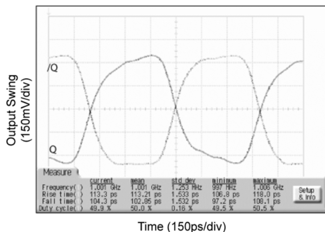
1GHz Output
