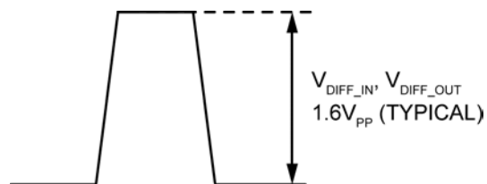
Figure 2. Differential Swing
