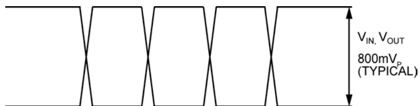
Figure 1. Single-Ended Swing
