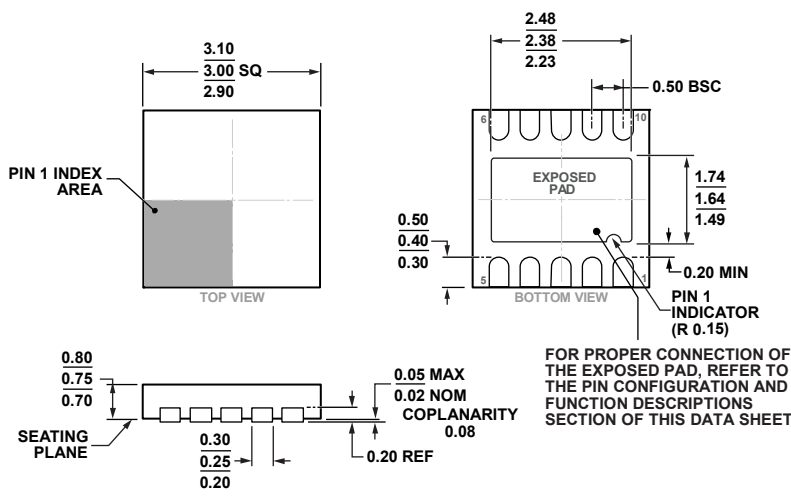
Figure 68. 10-Lead Lead Frame Chip Scale Package [LFCSP_WD] 3 mm × 3 mm Body, Very Very Thin, Dual Lead (CP-10-9) Dimensions shown in millimeters
