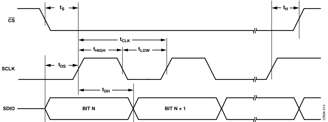
Figure 29. Serial Control Port Timing—Write
