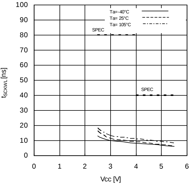
Figure 16. SCK Low Time vs Supply Voltage
