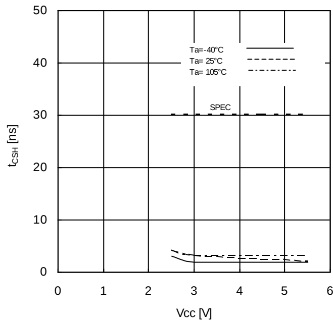
Figure 19. CSB Hold Time vs Supply Voltage
