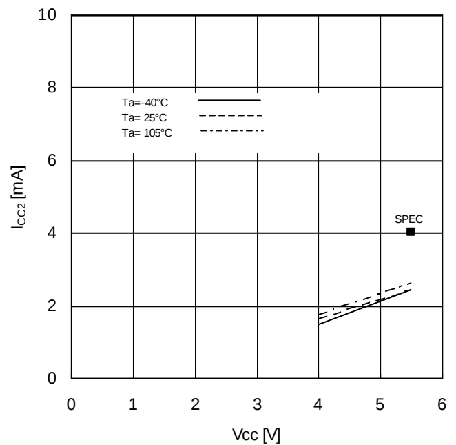
Figure 12 Supply Current (Read) vs Supply Voltage ( f_{SCK}=10\text{MHz} )
