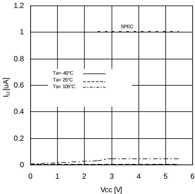
Figure 9. Input Leakage Current vs Supply Voltage (CSB, SCK, SI, HOLDB, WPB)
