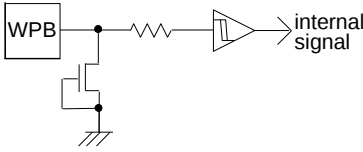
Figure 51. WPB input equivalent circuit
