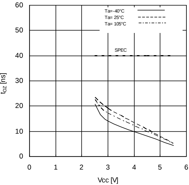
Figure 23. Output Disable Time vs Supply Voltage
