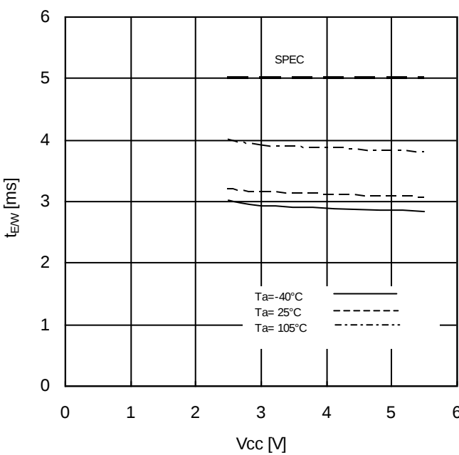
Figure 30. Write Cycle Time vs Supply Voltage
