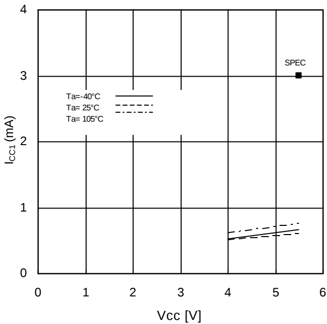
Figure 11. Supply Current (Write) vs Supply Voltage ( f_{SCK}=10\text{MHz} )
