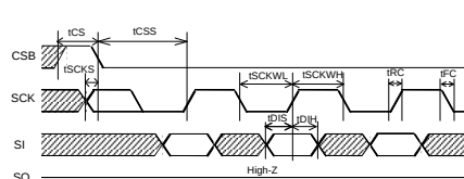
Figure 2-(a). Input timing
