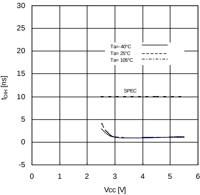
Figure 21. SI Hold Time vs Supply Voltage
