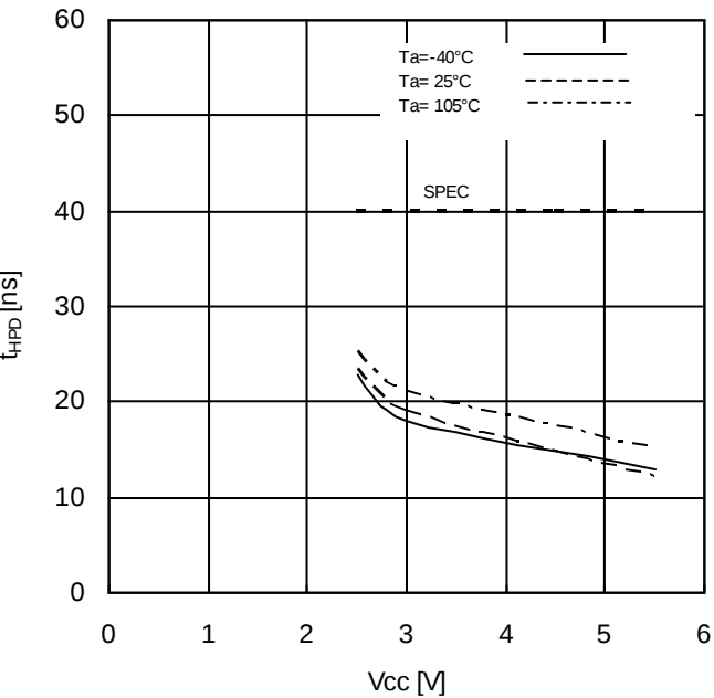
Figure 27. Time from HOLDB to Output change vs Supply Voltage
