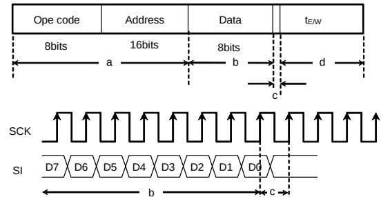
Figure 40. WRITE cancel valid timing
