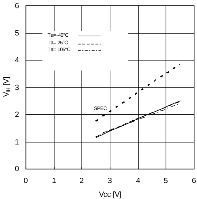
Figure 5. Input High Voltage vs Supply Voltage (CSB,SCK,SI,HOLDB,WPB)
