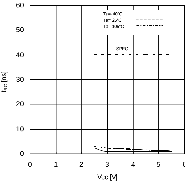
Figure 28. OUTPUT Rise Time vs Supply Voltage
