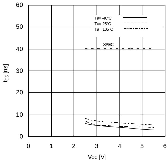
Figure 17. CSB High Time vs Supply Voltage
