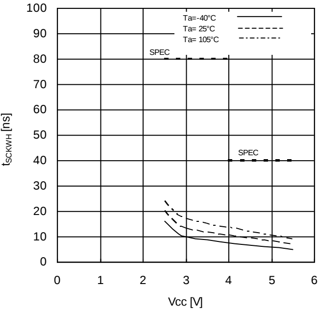
Figure 15. SCK High Time vs Supply Voltage
