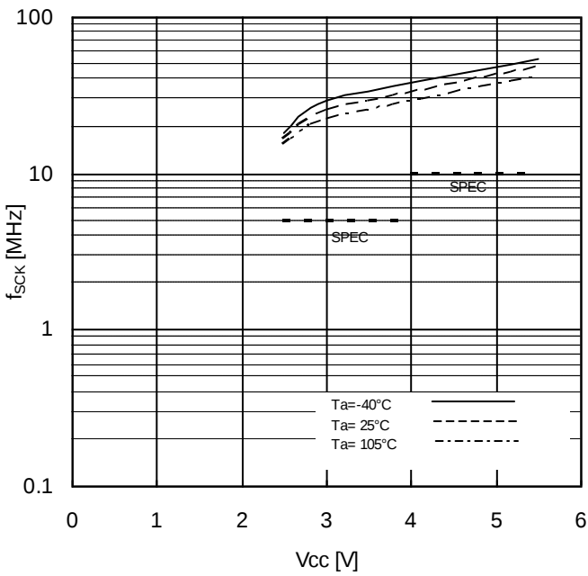
Figure 14. SCK frequency vs Supply Voltage
