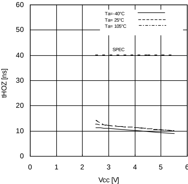
Figure 26. Time from HOLDB to Output High-Z vs Supply Voltage
