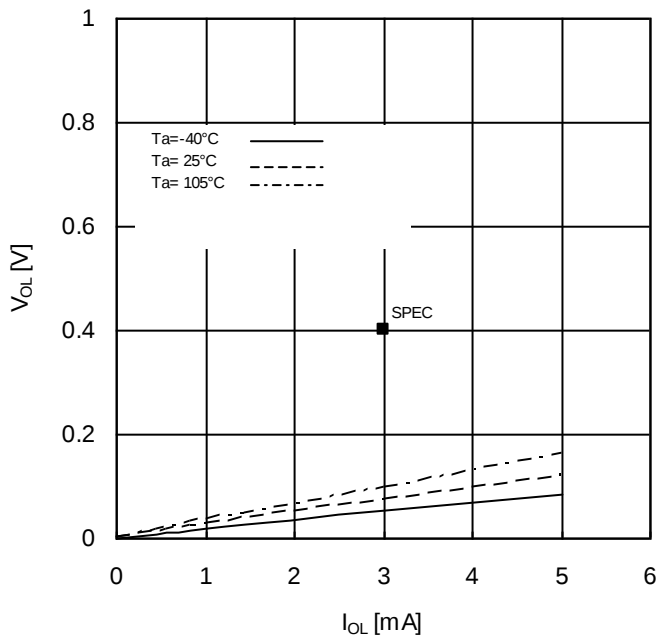
Figure 7 Output Low Voltage vs Output Current (V CC =2.5V)
