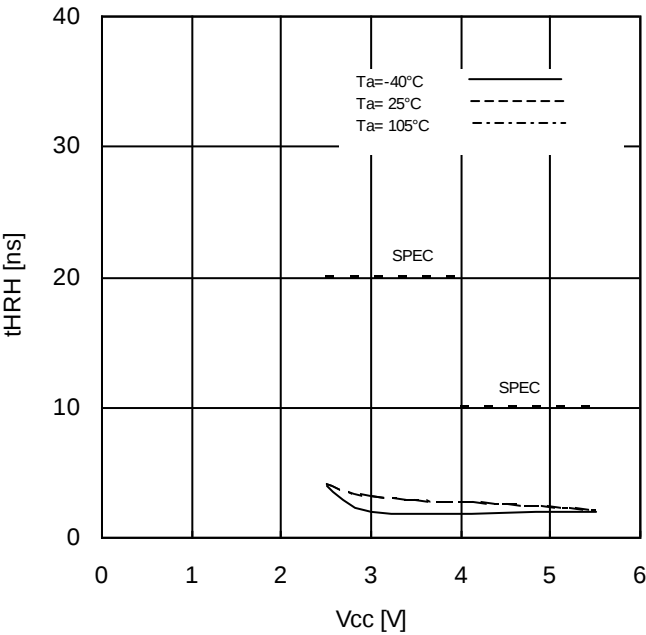
Figure 25. HOLDB Release Hold Time vs Supply Voltage
