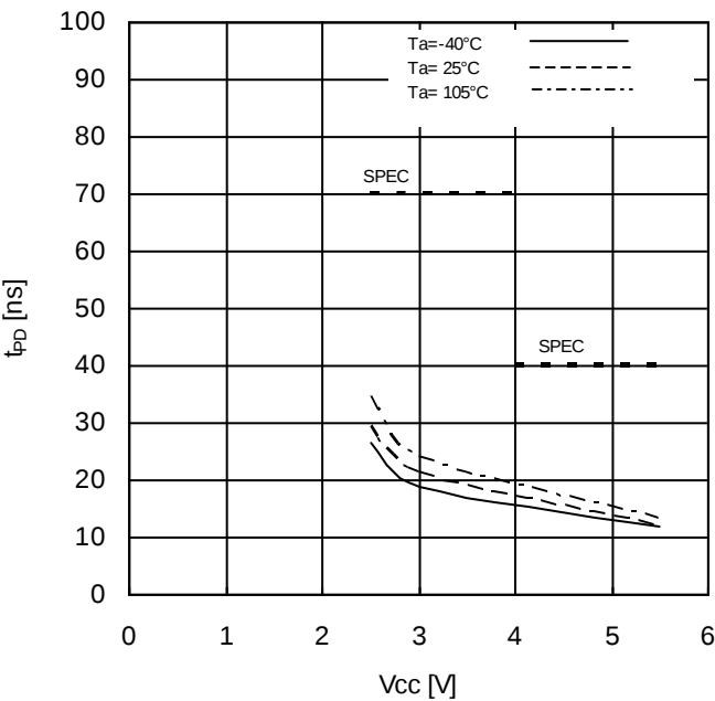
Figure 22. Data Output Delay Time vs Supply Voltage
