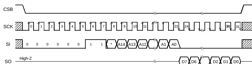
Figure 33. Read command
