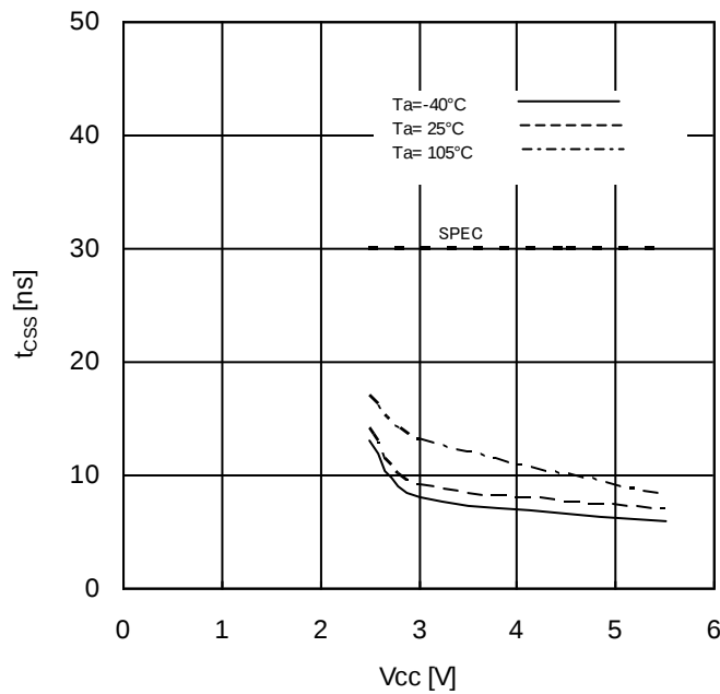
Figure 18. CSB Setup Time vs Supply Voltage
