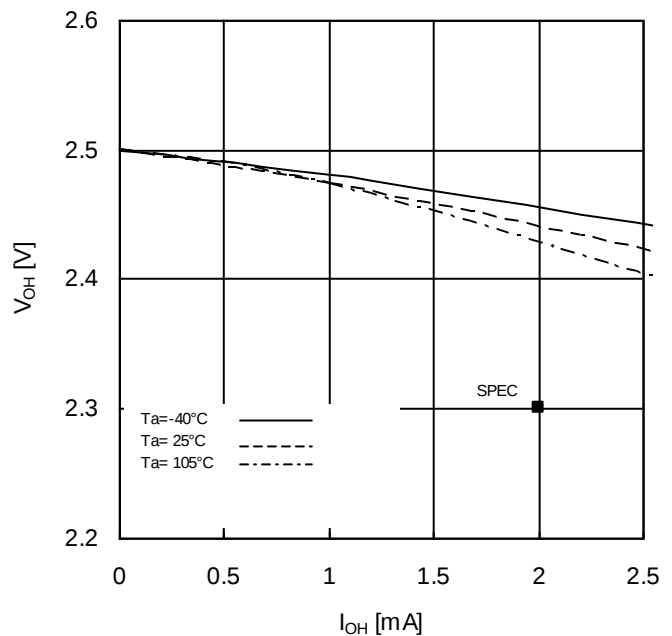
Figure 8. Output High Voltage vs Output Current (V CC =2.5V)
