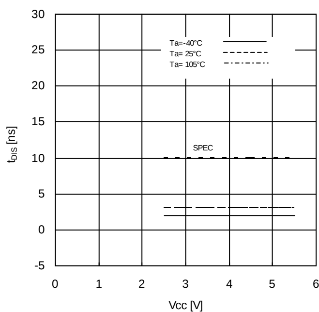
Figure 20. SI Setup Time vs Supply Voltage
