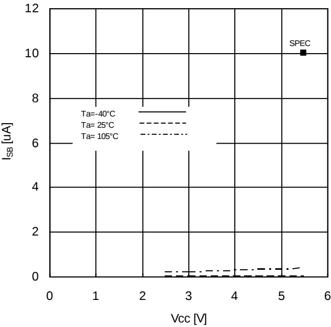
Figure 13. Standby Current vs Supply Voltage
