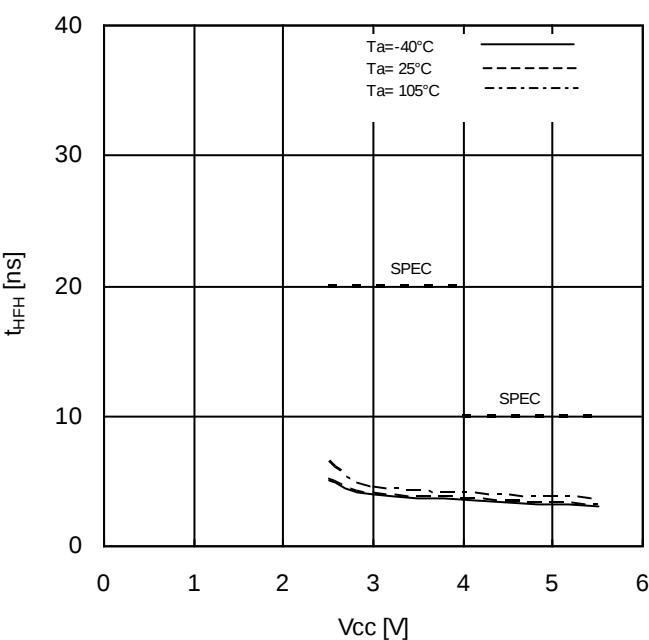
Figure 24. HOLDB Setting Hold Time vs Supply Voltage
