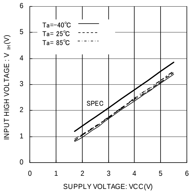
Figure 4. Input high voltage V_{IH} (CS, SK, DI, ORG)
