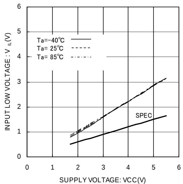
Figure 5. Input low voltage V_{IL} (CS, SK, DI, ORG)
