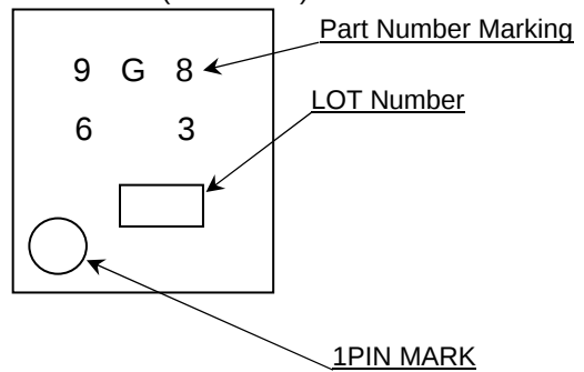
TSSOP-B8J(TOP VIEW)
