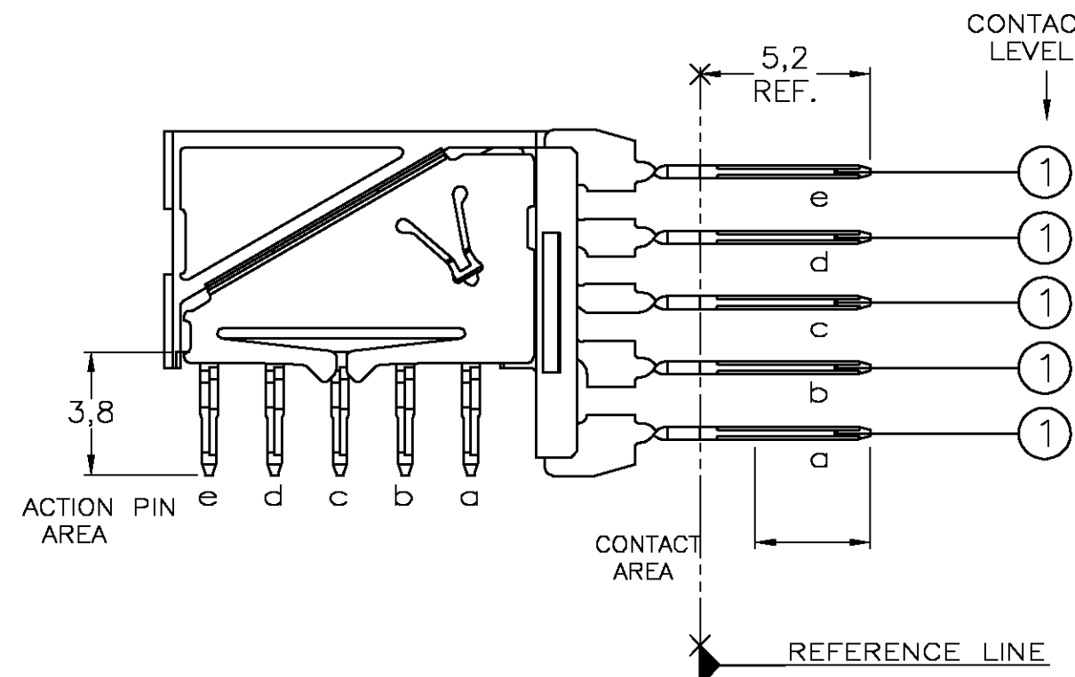
CONTACT DIMENSIONS
