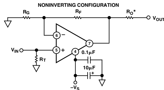
Figure 7. Inverting and Noninverting Configurations
