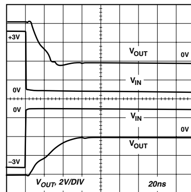
TPC 34. Overdrive Recovery; V_S = \pm 5\text{ V} , G = +2 , R_F = 750\text{ }\Omega , R_L = 100\text{ }\Omega , V_{IN} = 3\text{ V p-p} ( T = 1\text{ }\mu\text{s} )
