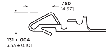
B Low Force (6.5 Amp Max. Current Rating)
