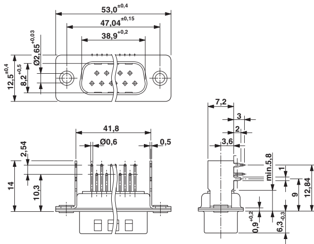
Dimensioned drawing
