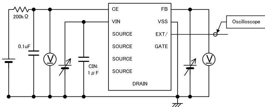
Circuit
