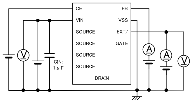
Circuit
