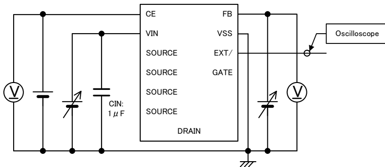
Circuit
