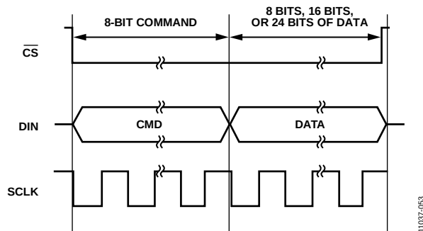
Figure 26. Writing to a Register (8-Bit Command with Register Address Followed by Data of 8, 16, or 24 Bits; Data Length Is Dependent on the Register Selected)
