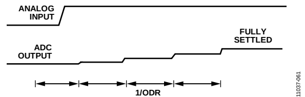
Figure 37. Step Input Without Single Cycle Settling
