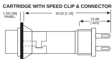
CARTRIDGE WITH SPEED CLIP & CONNECTOR
