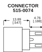
CONNECTOR 515-0074
