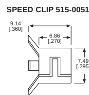
SPEED CLIP 515-0051
