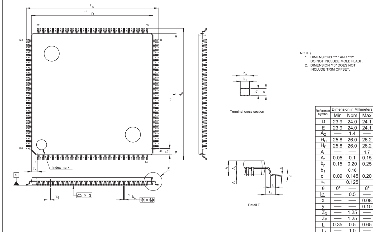
Figure C 176-Pin LQFP (PLQP0176KB-A)
