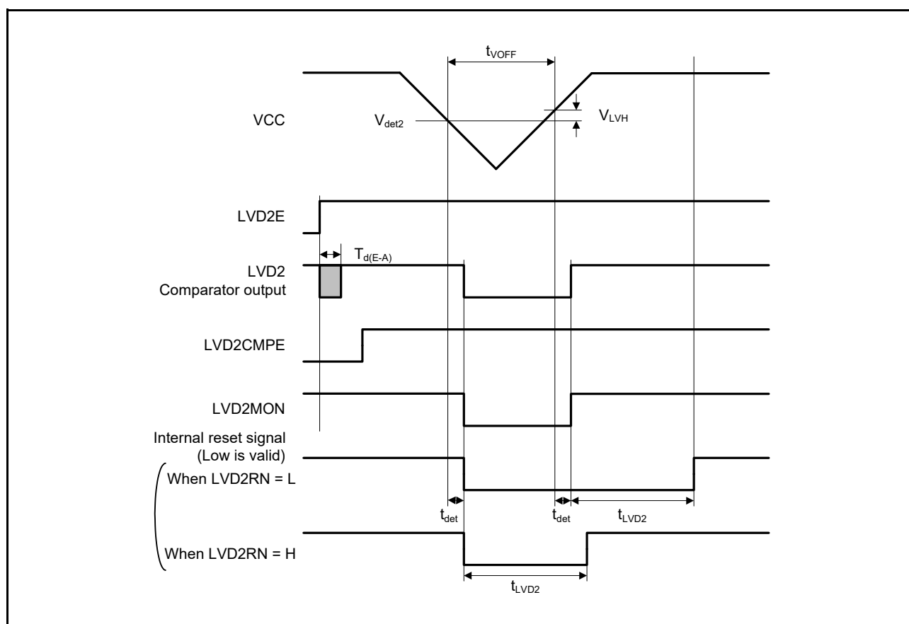
Figure 5.86 Voltage Detection Circuit Timing ( V_{\text{det2}} )
