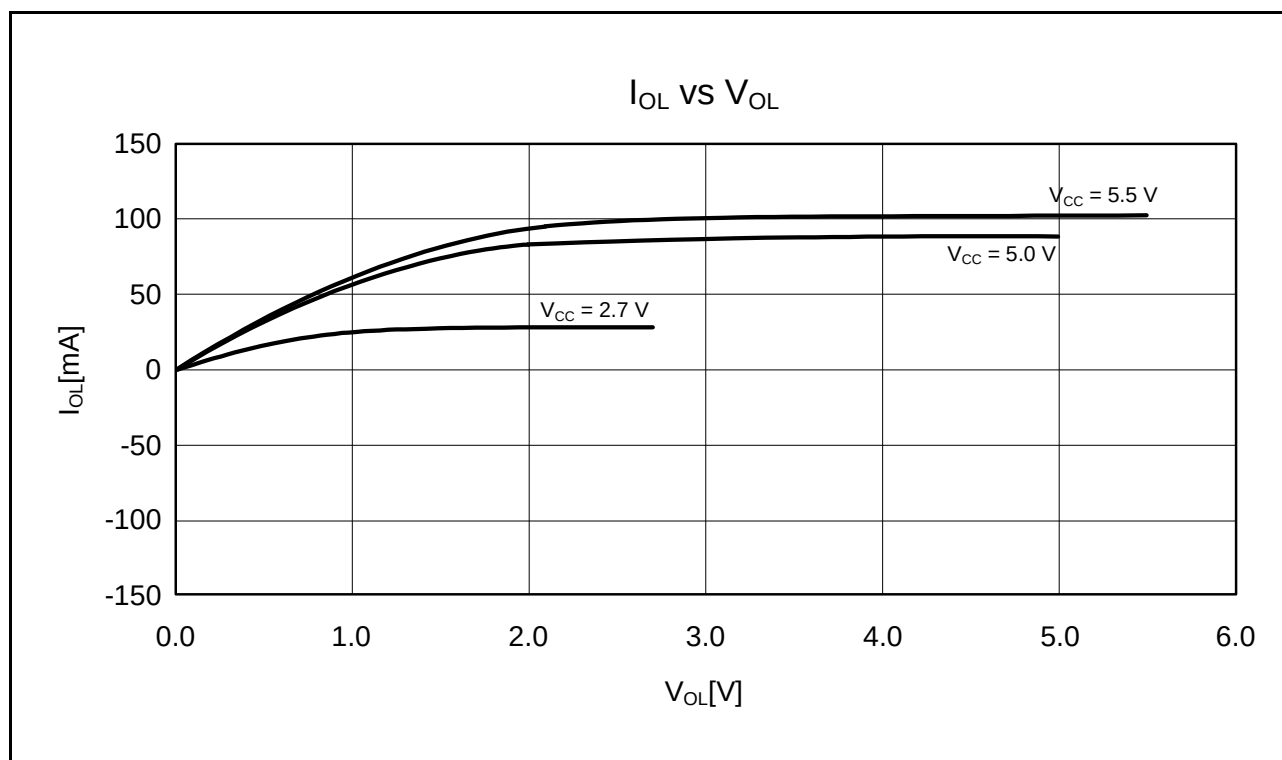
Figure 5.16 V_{OL} and I_{OL} Voltage Characteristics of RIIC Output Pin at T_a = 25^\circ\text{C} (Reference Data)
