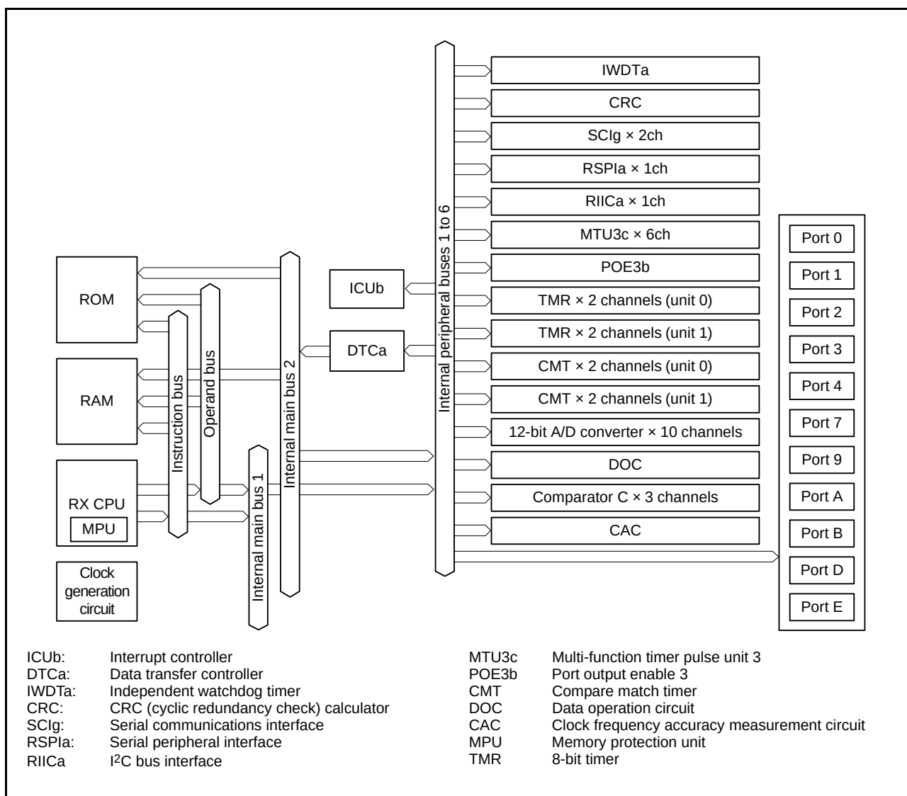
Figure 1.2 Block Diagram
