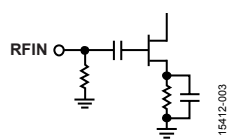
Figure 6. RFIN Interface Schematic
