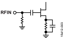
Figure 6. RFIN Interface Schematic
